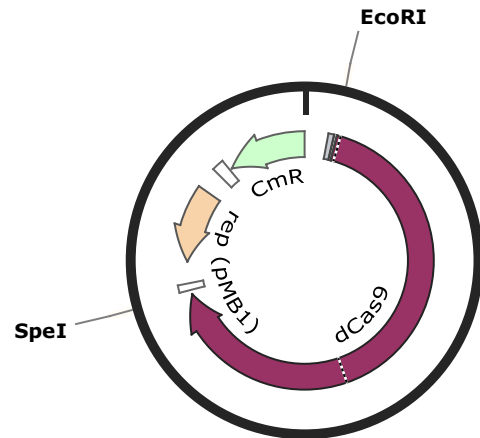
pSB1C3_dCas9QC 6193 bp
