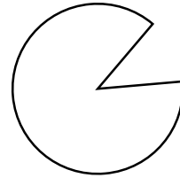
Beta galactosidase
