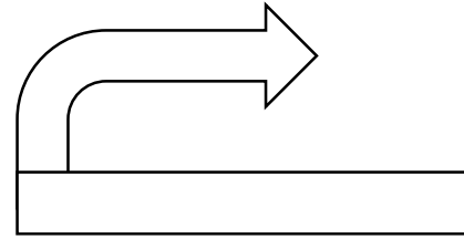
Promoter
