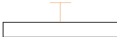
Terminator
