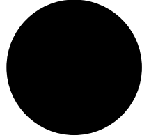
Colour
