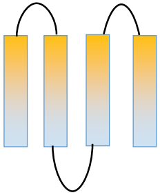
Recombinant receptor
