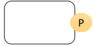
Transcription factor
