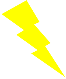
Light
