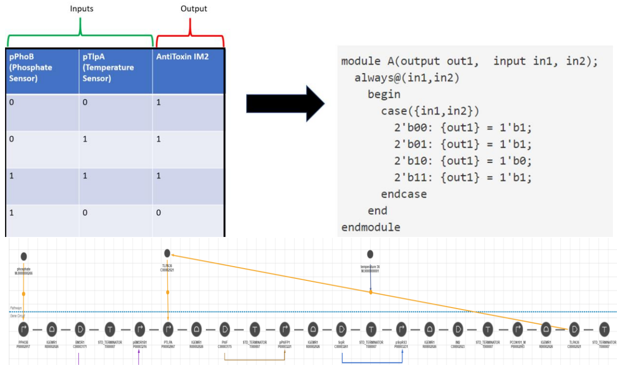
Figure 10 (Above) Converting the logic table to Verilog Code so that Cello can generate a circuit design. (Below) The Automated Circuit generated from Cello as displayed using AdvanceSyn
